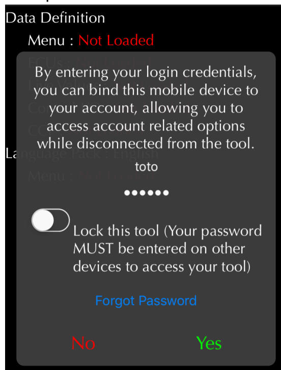
Figure 2. Tool Binding
