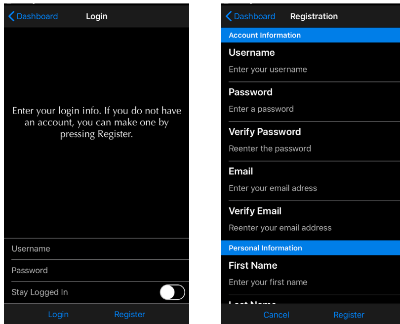
Figure 1. Registering
